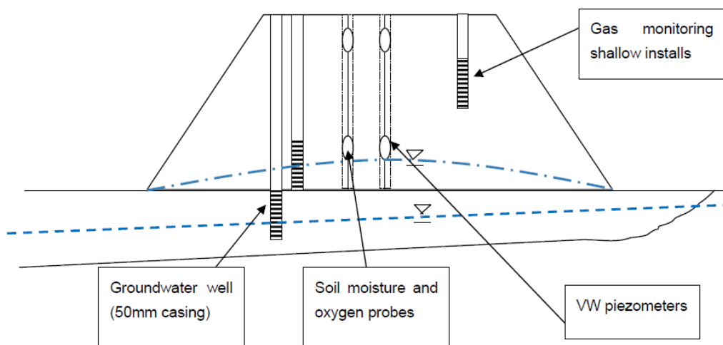
Fig. 3. Conceptual layout of monitoring equipment
