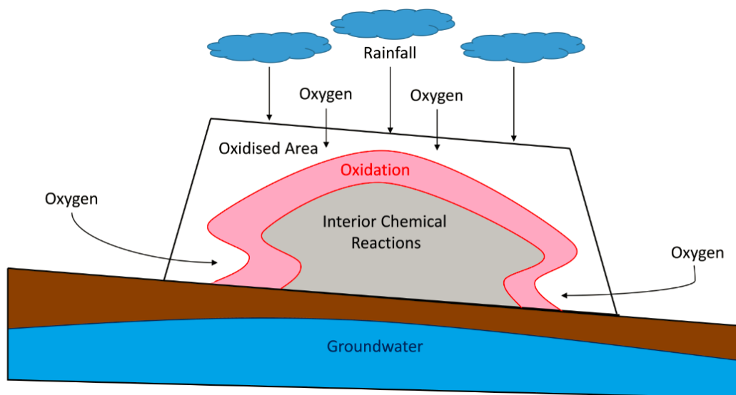
Fig. 1. Generic model of AMD production and contaminant migration from a waste rock dump after Ritchie 1994
