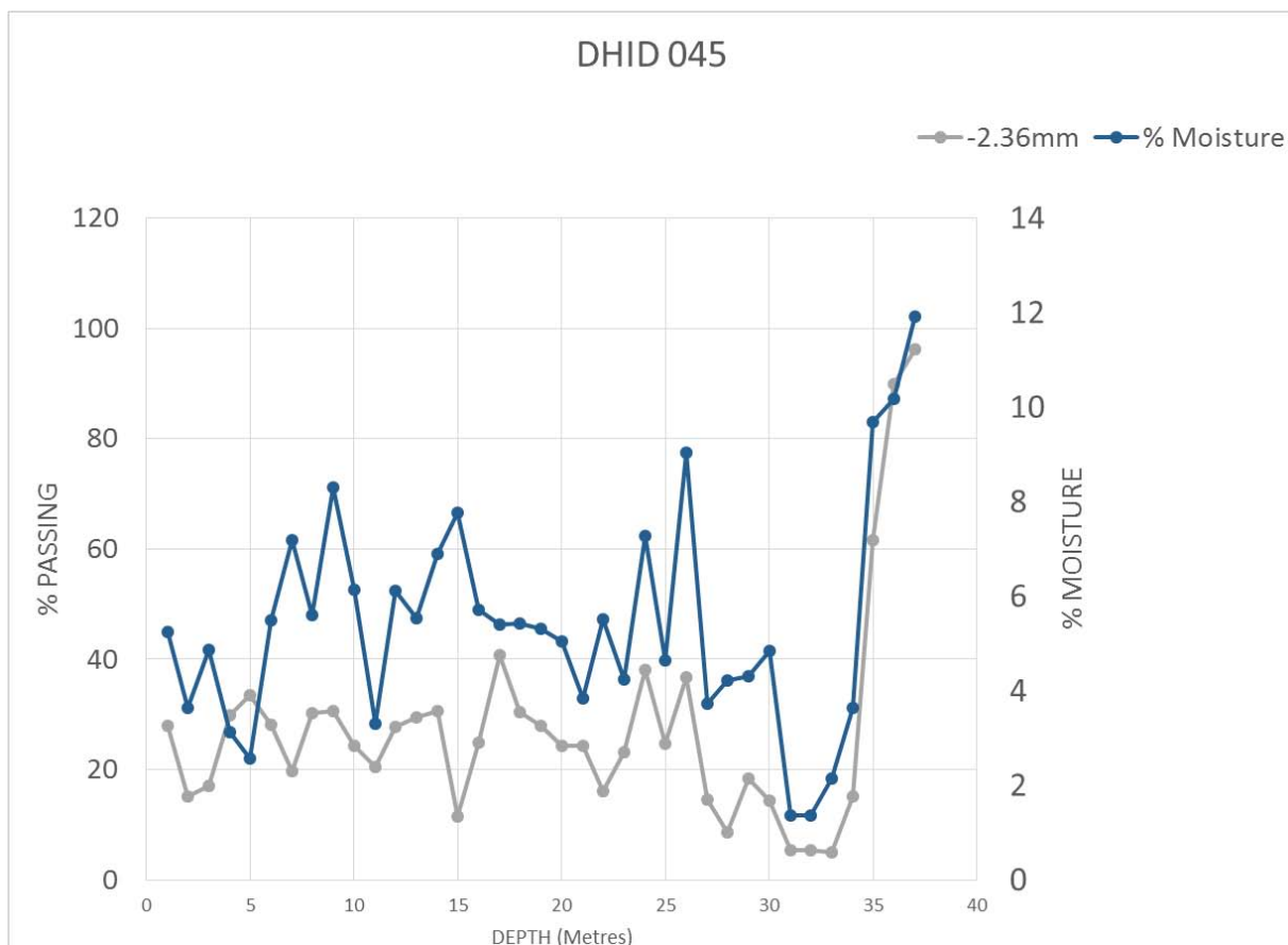
Fig. 4. Typical moisture content, grain size profile though waste dump
